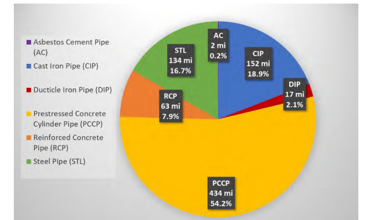
Figure 12. Transmission system inventory by material
