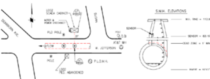
Figure 64. Example of a level sensor at West Jefferson and Sloan
