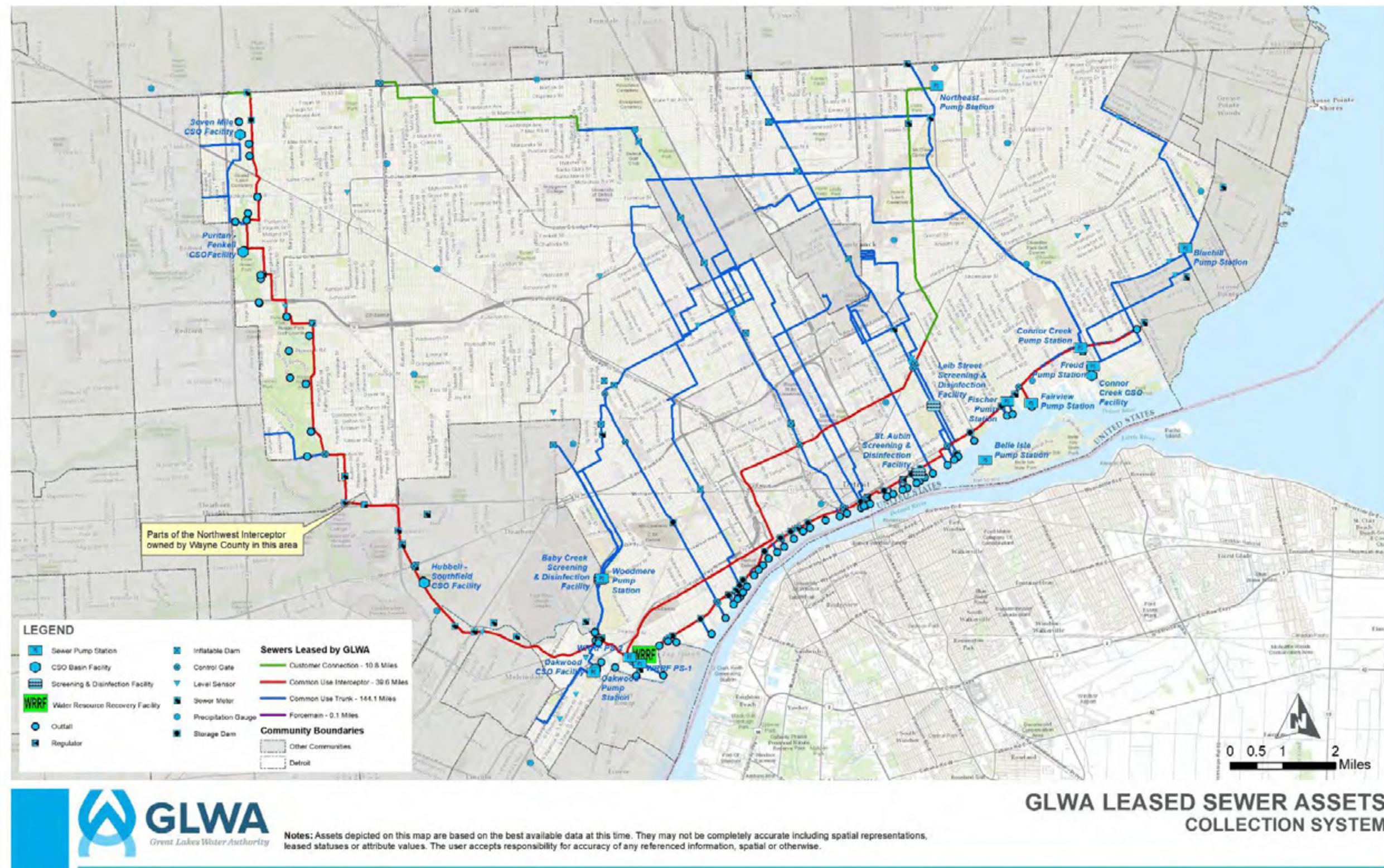
Figure 51. Sewer interceptors and trunk sewers operated/maintained by GLWA
