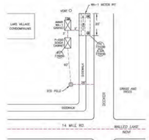
Figure 17. Pressure Monitoring Site at 14 Mile and Decker
