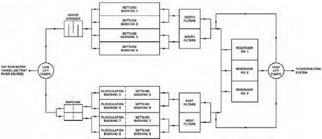
Figure 9. Springwells WTP process diagram
