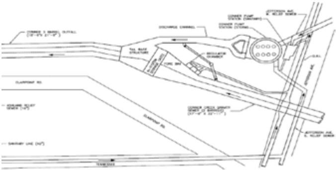
Figure 56. Schematic of Conner Creek Pump Station
