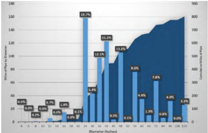
Figure 13. Transmission system inventory by diameter
