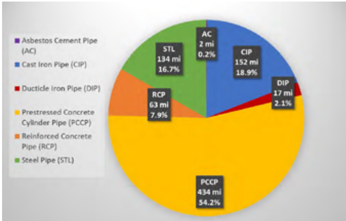
Figure 12. Transmission system inventory by material
