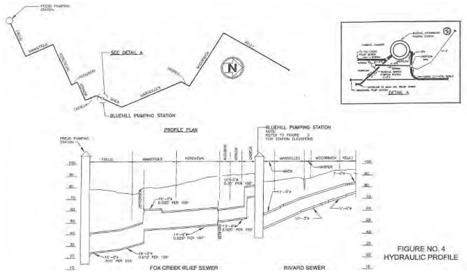
Figure 54. Hydraulic Profile at Bluehill Station
