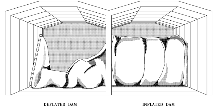
Figure 65. Inflatable dam illustration
